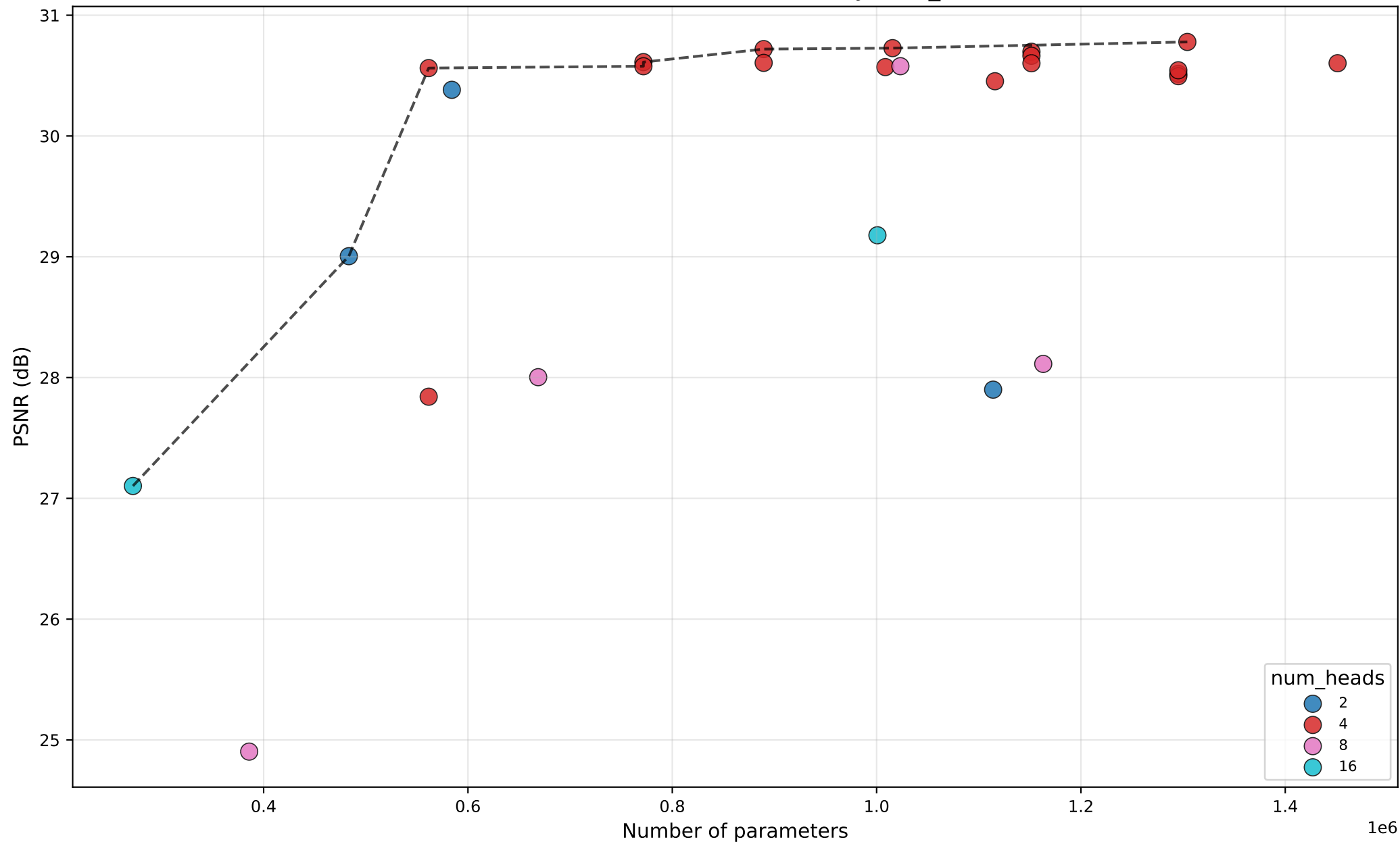
PSNR vs #Params — OmniSR — by num_heads
